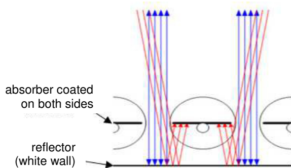
Figure 3: Path of irradiation on power tube collector and different sun positions
